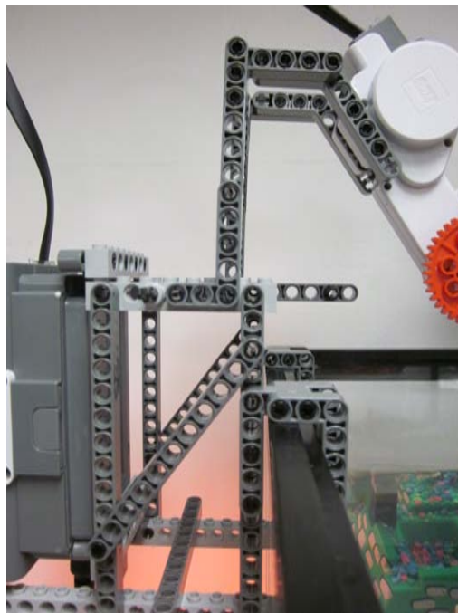
(Tank Gripper)
